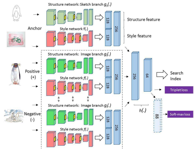
Figure 2. Hierarchical triplet convnet combining vectors from the style (Fig. 1) and structure [4] streams. Joint embedding of the two modalities is learned (Sec. 3.2.3) from the concatenated features initially via classification loss, followed by hard negative mining resulting in a 64-D descriptor for indexing.
